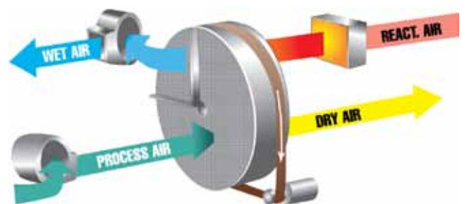
Desiccant dehumidifier
